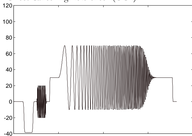
“Ghost Cancelling Reference” (GCR):
