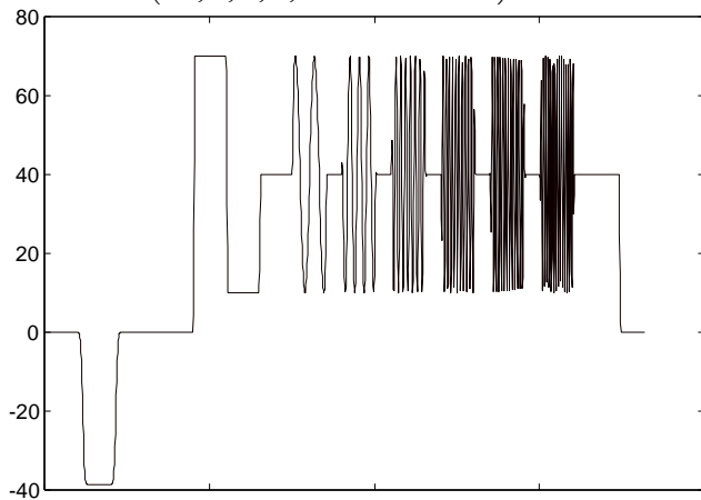
Multiburst (0.5, 1, 2, 3, 3.58 e 4.2 MHz):
