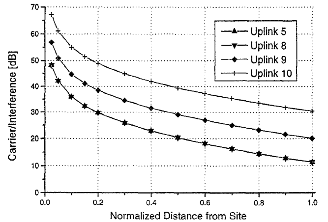
Figure 4: Carrier-to-interference ratio as a function of normalized distance for the uplink
