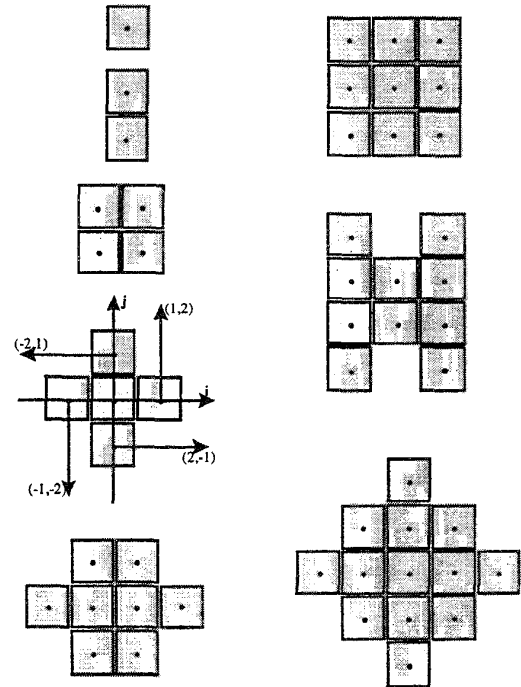
Figure 2: Some possible reuse patterns ( N = 1, 2, 4, 5, 8, 9, 10, 13 microcells per cluster)
