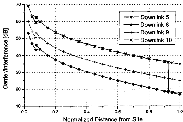
Figure 5: Carrier-to-interference ratio as a function of normalized distance for the downlink
