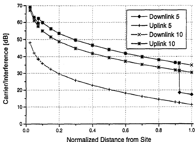
Figure 6: Carrier-to-interference ratio as a function of normalized distance for up and downlinks compared.
