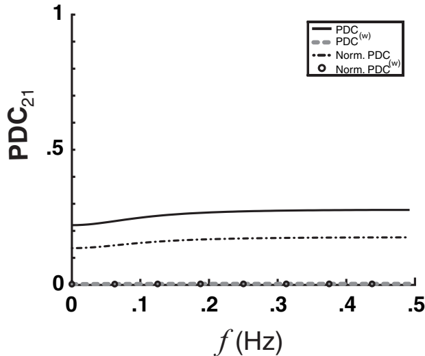
Fig. 2. Comparison between PDC and PDC^{(w)} with and without time-series data pre-normalization.
