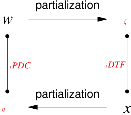
Figure 1: The diagram summarizes the relationship between the various descriptive processes associated with the original observations \mathbf{x} including the innovations process \mathbf{w} and their respective partialized versions \boldsymbol{\eta} and \boldsymbol{\zeta} . The mutual information rate relationships are described by \iota PDC for (\boldsymbol{\eta}, \mathbf{w}) and \iota DTF for (\boldsymbol{\zeta}, \mathbf{x}) . Information flow sources are indexed by the greek type face vector components and the information receiving structures are chosen among the components of the latin type face processes.
